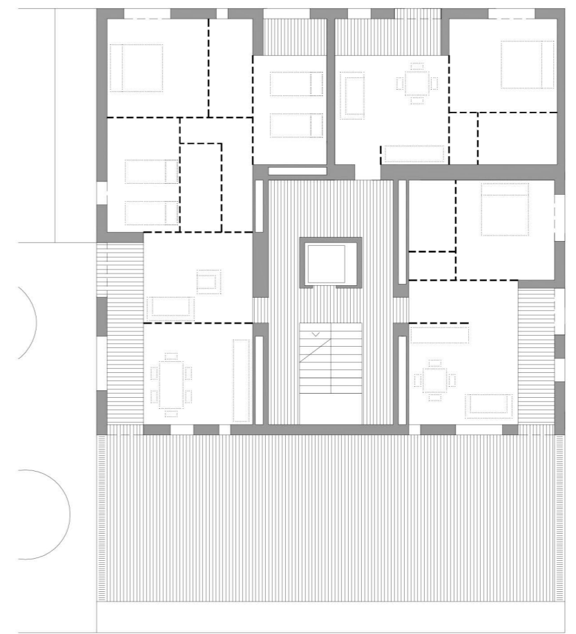
PIANO INTERMEDIO
